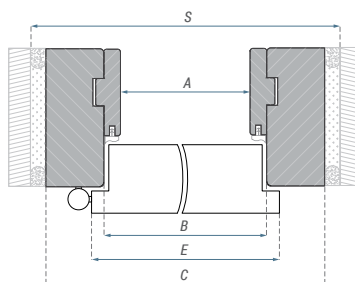
Dimensions of FIRE wooden fixed and adjustable door frame [mm]:
