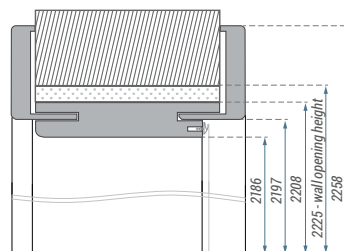
▼ Dimensions of door frame for Natura HB PN22 door.
