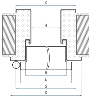
Dimensions of FIRE steel fixed door frame [mm]:
