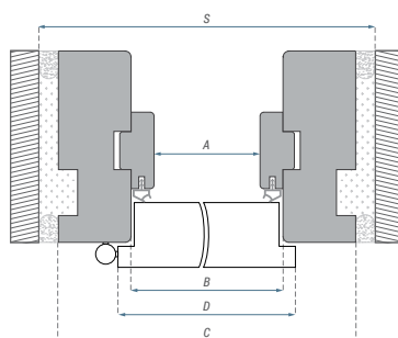
Dimensions of BORD MDF door frame [mm]:
